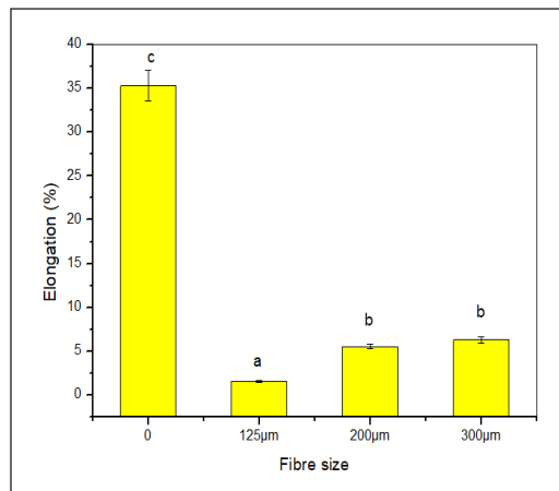
Figure 6. The tensile strain of coconut fibre composition with different fibre sizes (MPa)
