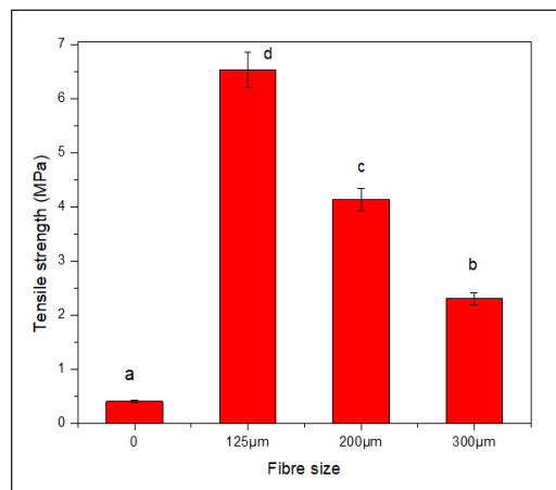
Figure 4. Tensile strength of coconut fibre composites with different fibre sizes (MPa)
